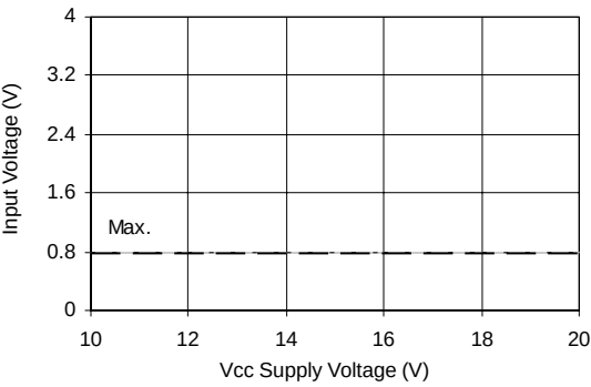
Figure 13B. Logic "0" ( \overline{HIN} ) & Logic "1" ( \overline{LIN} ) Input Voltage vs Voltage
