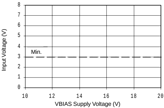
Figure 12B. Logic "1" ( \overline{HIN} ) & Logic "0" ( \overline{LIN} ) Input Voltage vs Voltage
