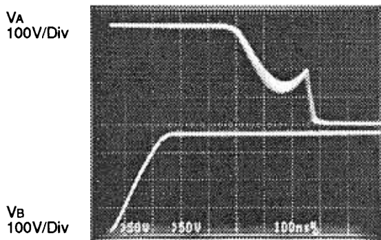
Fig 16. - Non-ZVT Operation
