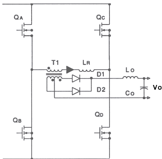
Fig 1. - Full Bridge Topology - General Circuit
