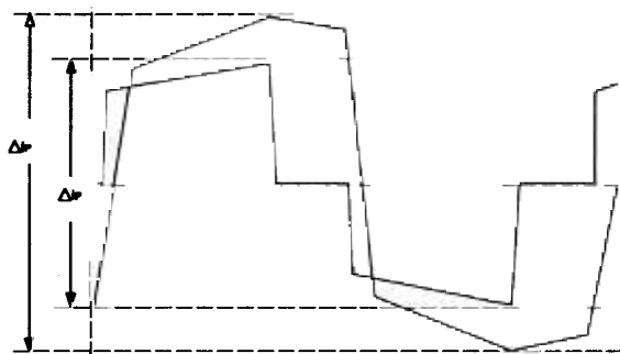
Fig 13. - Primary Current - ZVT vs Square Wave
