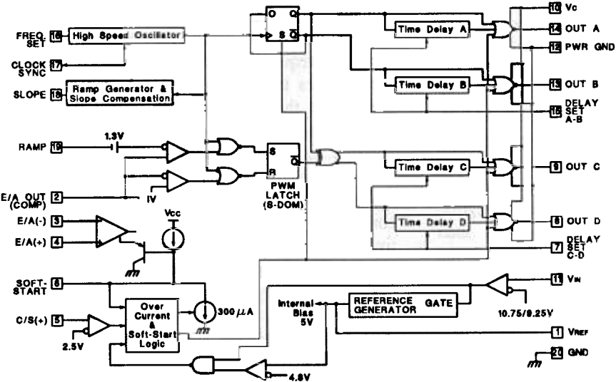
Fig 14. - UC3875 Block Diagram
