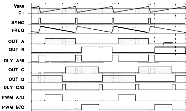
Fig 3. - Phase Shifted PWM Control Waveforms
