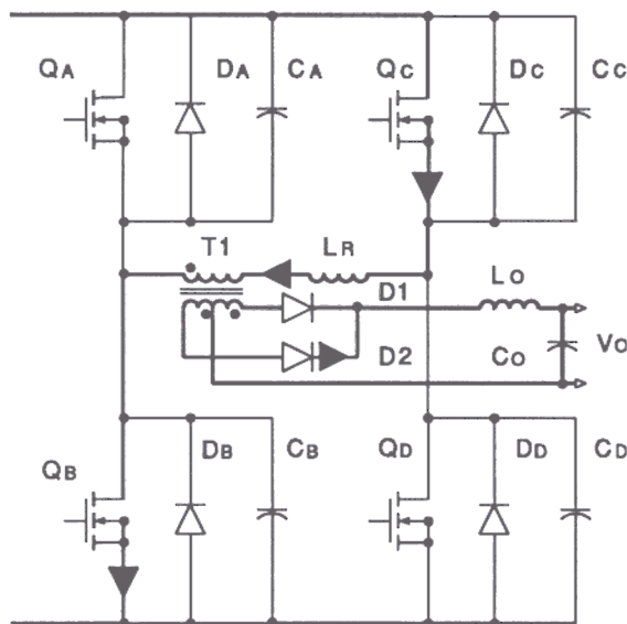
Fig 11. - Power Transfer Interval
