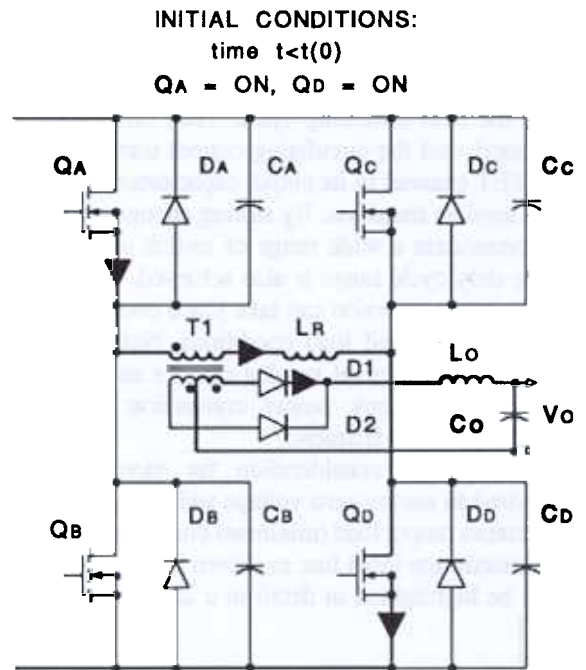
Fig 7. - Initial Conditions
