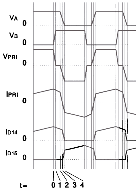
Fig 12. - Operational Waveforms
