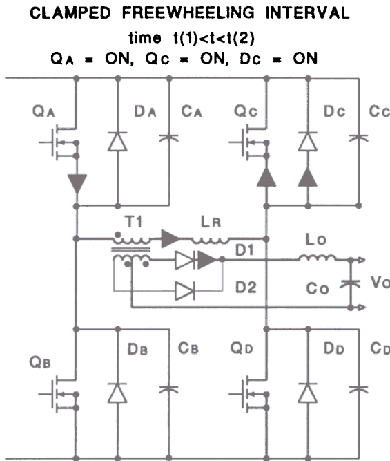
Fig 9. - Clamped Freewheeling Interval
