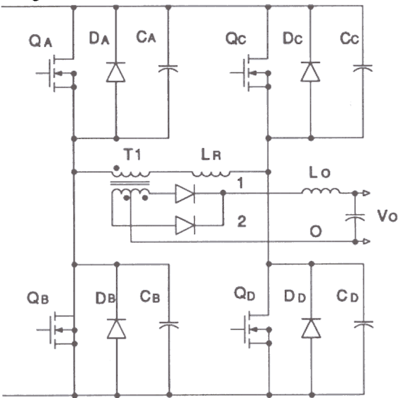
Fig 5. - Phase Shifted PWM Switch Orientation
