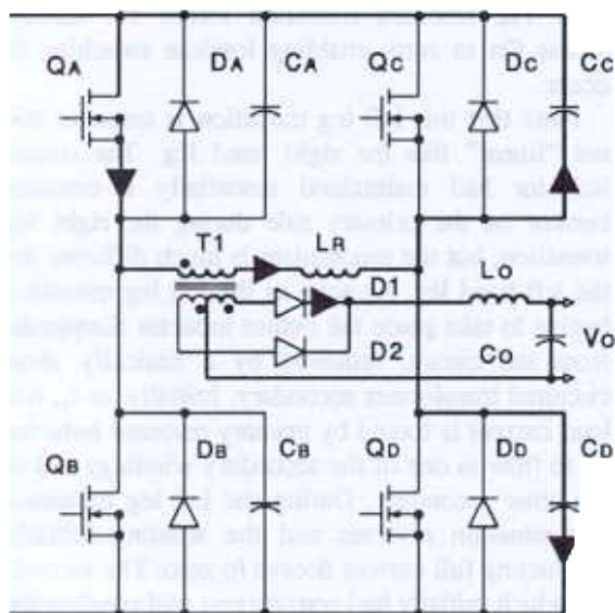
Fig 8. - Right Leg Transition
