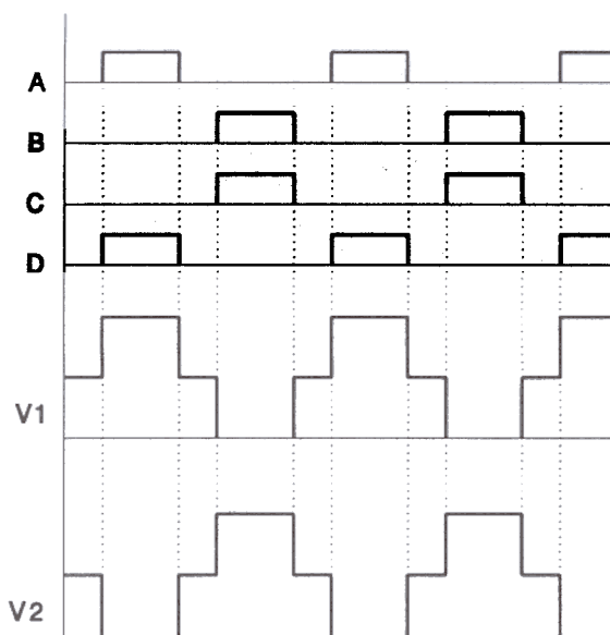
Fig 2. - Conventional Full Bridge Waveforms
