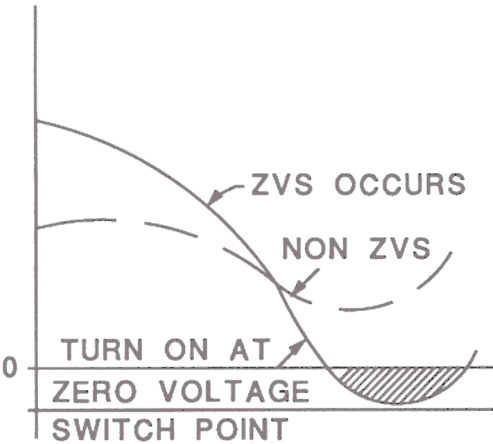
Fig 4. - ZVS Limitations
