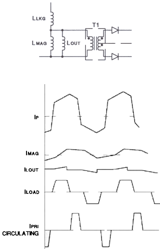
Fig 6. - Primary Magnetic Components
