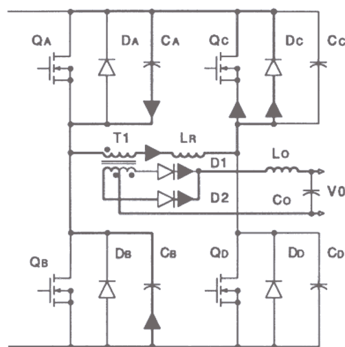
Fig 10. - Left Leg Transition
